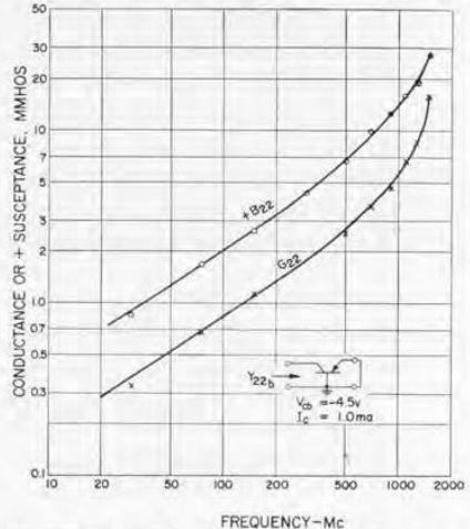
Figure 10. Plot of short-circuit output admittance as a function of frequency for a diffused-base transistor.
