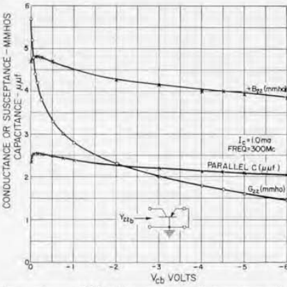
Figure 8. Variation of parameters of a diffused-base transistor as a function of collector voltage.
