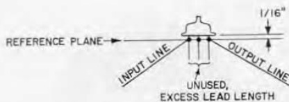
Figure 6. Sketch of connections to transistor, showing the reference points of measurement.
