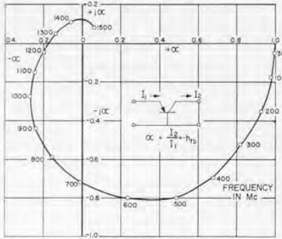
Figure 9. Plot of \alpha_1 or -h_{fb} versus frequency for a diffused-base transistor.
